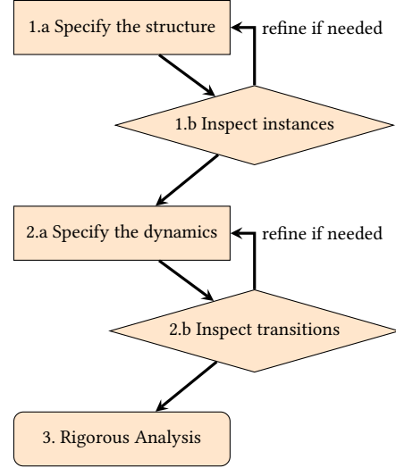
Figure 1. A customary workflow for modeling a software system in Alloy. Steps 1.a and 2.a correspond to user input in the form of model specification. In steps 1.b and 2.b, arbitrary model instances generated by Alloy are visually inspected by the users to identify and address any apparent flaws. In the final step, the Alloy analyzer automatically checks for all possible states and transitions within a given bound.
